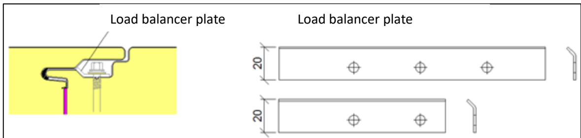
Figure 8. Tightening of screws on TENAX W sandwich panels with a hidden key (side joint H)
