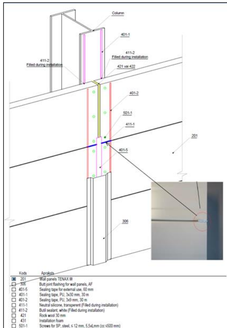
Figure 6. Sealing and strengthening of sandwich panels
