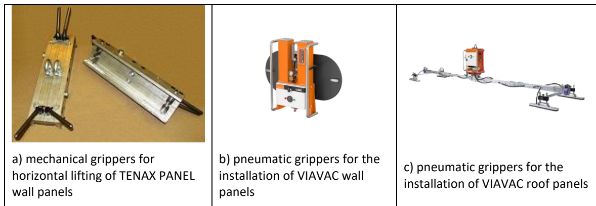
Figure3. Examples of gripping devices
