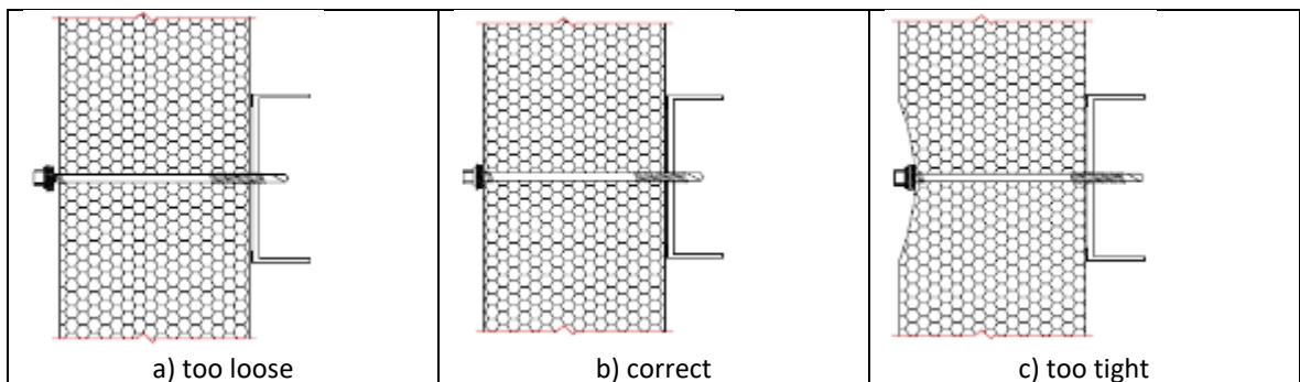
Figure 7. Tightening of screws on TENAX W sandwich panels with a standard key (side joint S or T)
