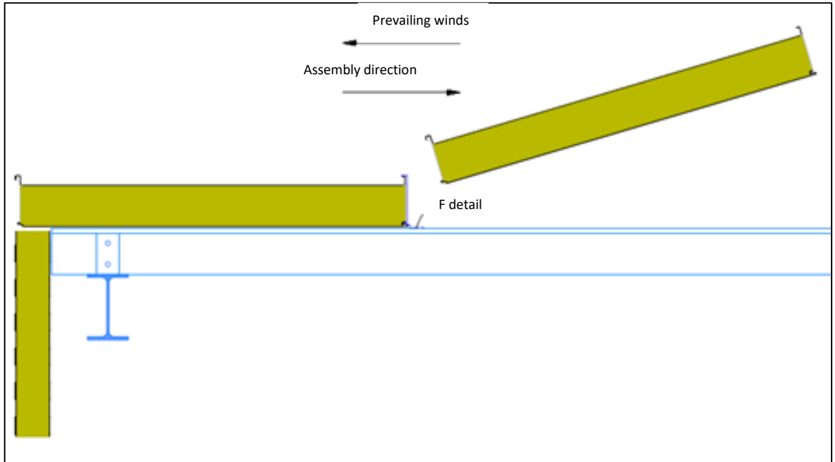
Figure 13. The recommended direction for the installation of roll-folded roof panels
