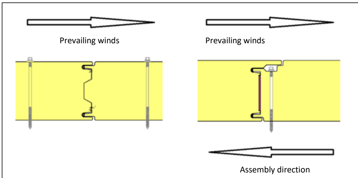
10. figure. The recommended direction for vertical installation
