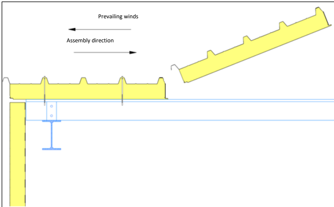
Figure 11. The recommended direction for installation of profiled roof panels
